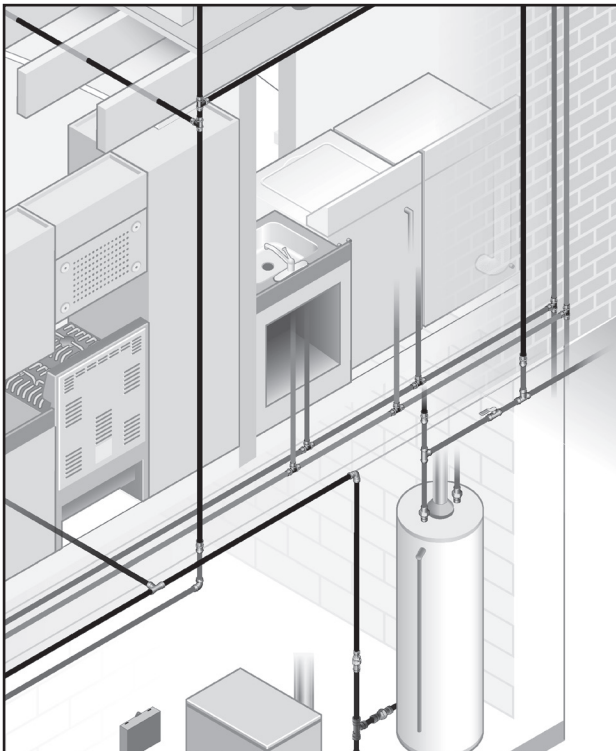
Branch-and-Tee Installation
