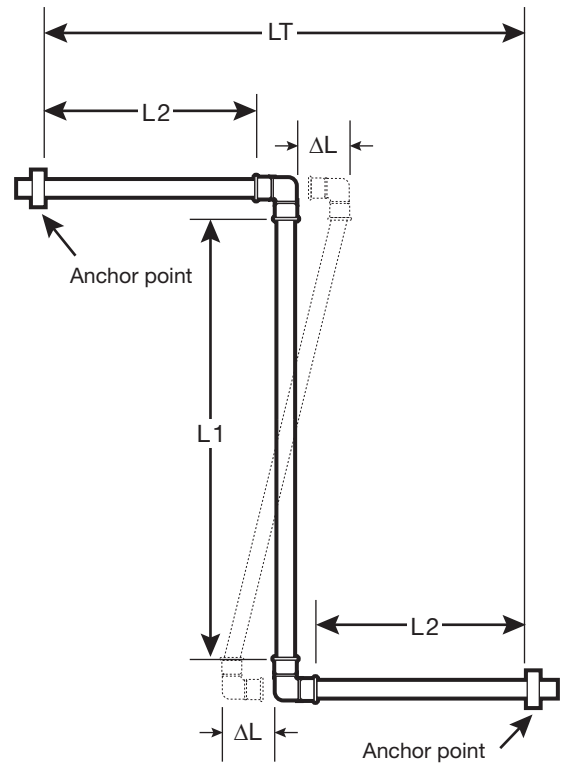
Z-type offset
