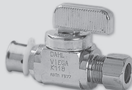
1/4-Turn Straight Stop Valve PureFlow Press to \frac{3}{8} " O.D. Riser
