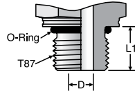
ISO 6149 Nonadjustable
