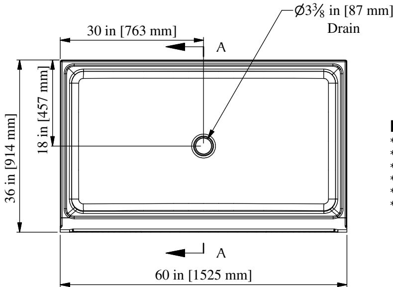
PLAN 60" [1525mm] x 36" [914mm] Shower Pan w/ 4" [101mm] Threshold
