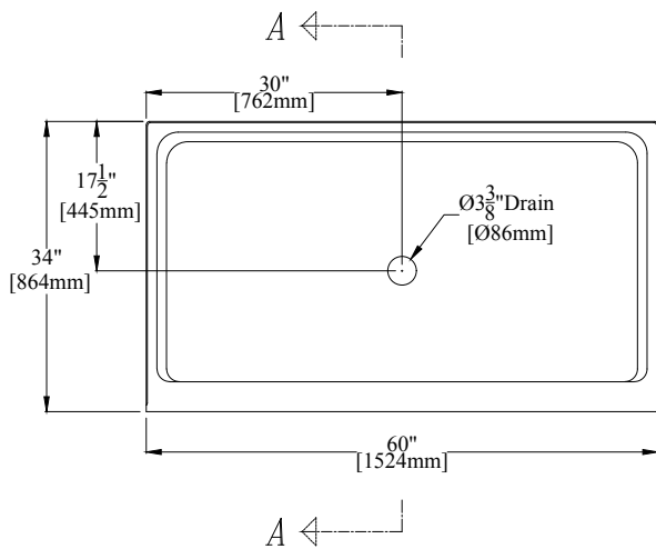
60" x 34" [1524mm x 864mm] Shower Pan w/ 6" [152mm] Threshold
