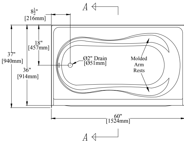
60" [1524mm] Bathtub w/ 20 1/2" [522mm] Apron, Molded Arm Rests, & Removable Access Panel
